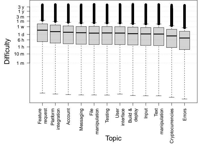
Fig. 4. Boxplot of D(GH_{i_t}) (difficulty of GitHub topics)
