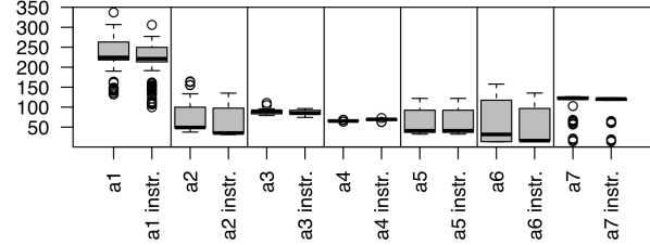
(b) Memory consumption of selected apps (in Mb)
